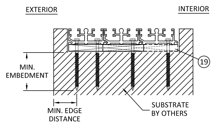
C 7 VERTICAL SECTION THROUGH FRAME - SILL
