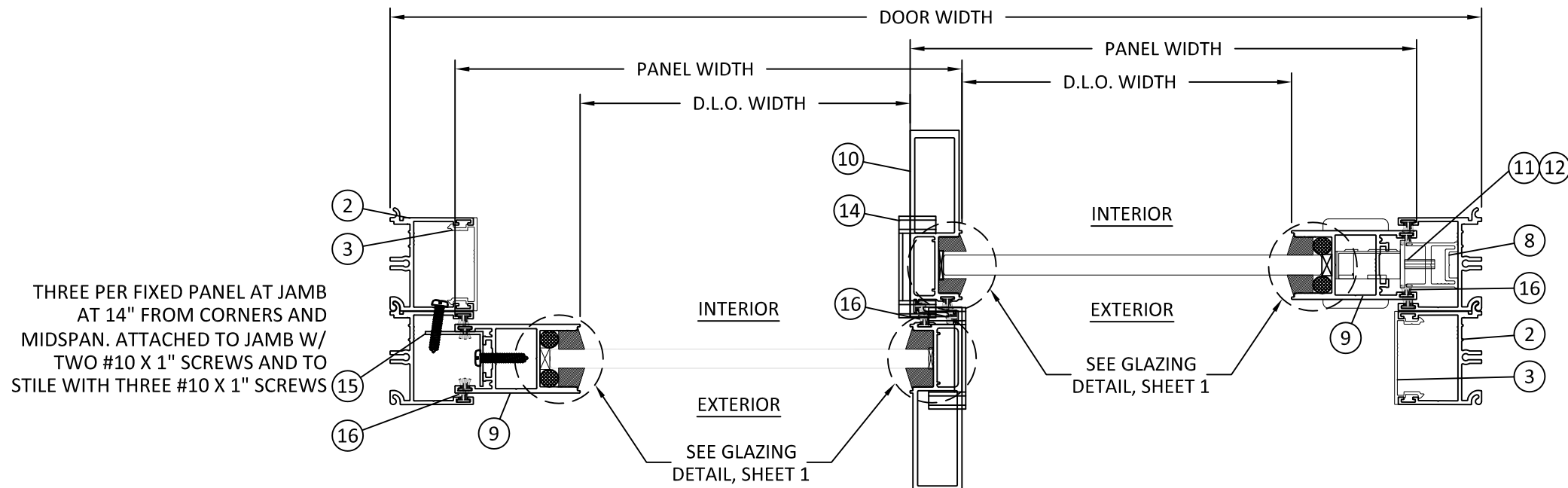
B 6 HORIZONTAL SECTION TWO PANEL - TWO TRACK
