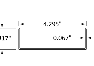
7 TWO TRACK DRAIN PAN 6063-T5 ALUMINUM
