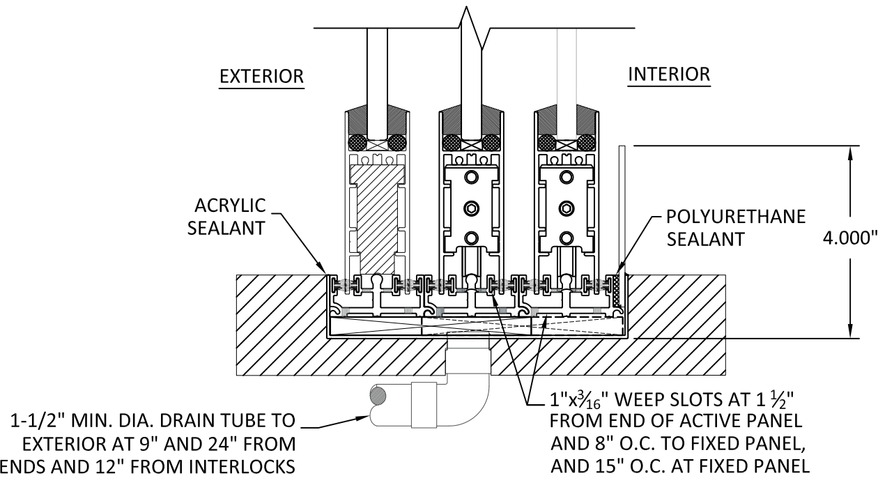
VERTICAL SECTION SILL DRAINAGE DETAIL
