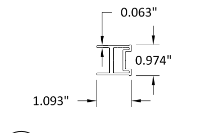
8 JAMB STILE ADAPTOR 6063-T5 ALUMINUM
