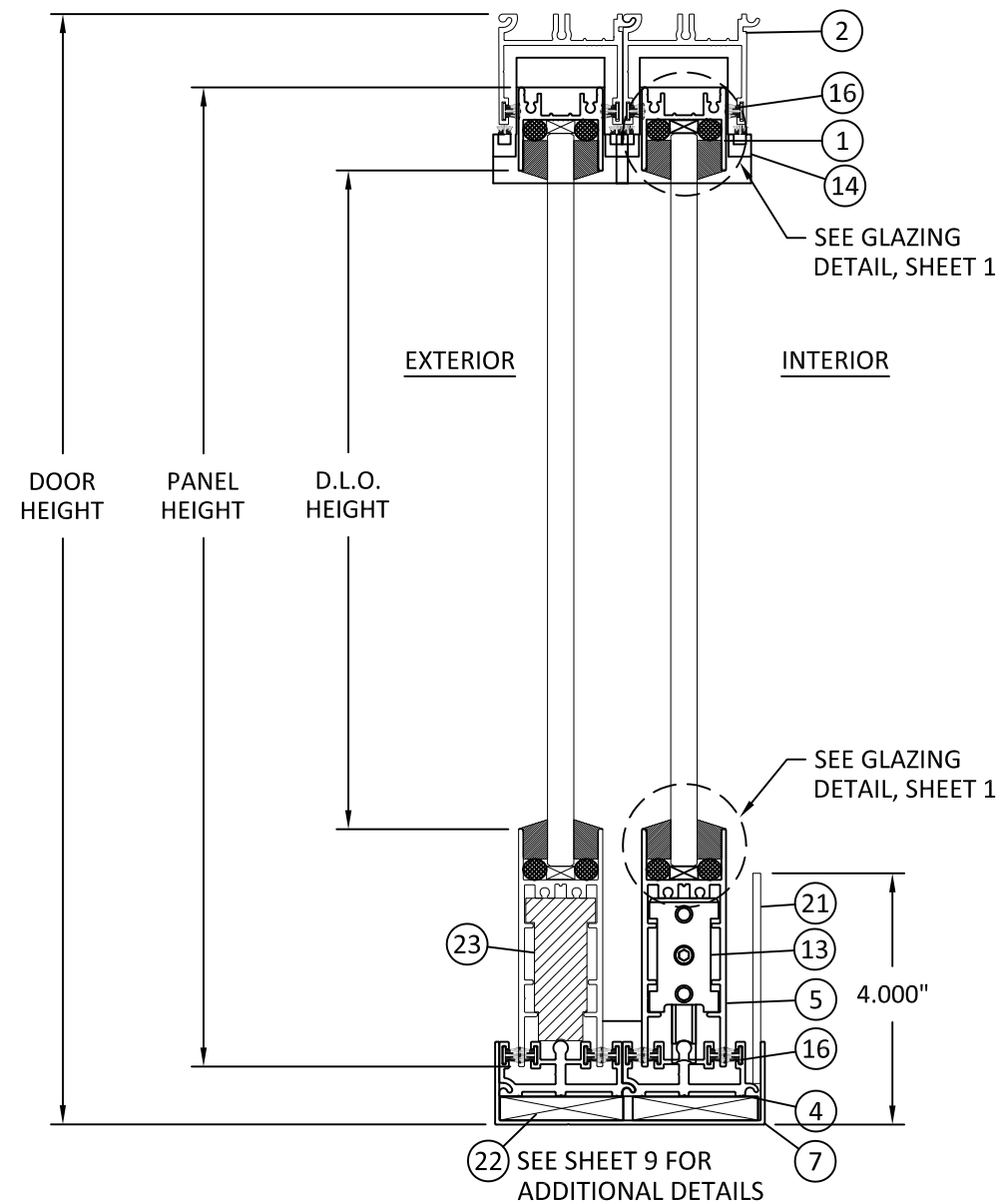
VERTICAL SECTION TWO PANEL - TWO TRACK
